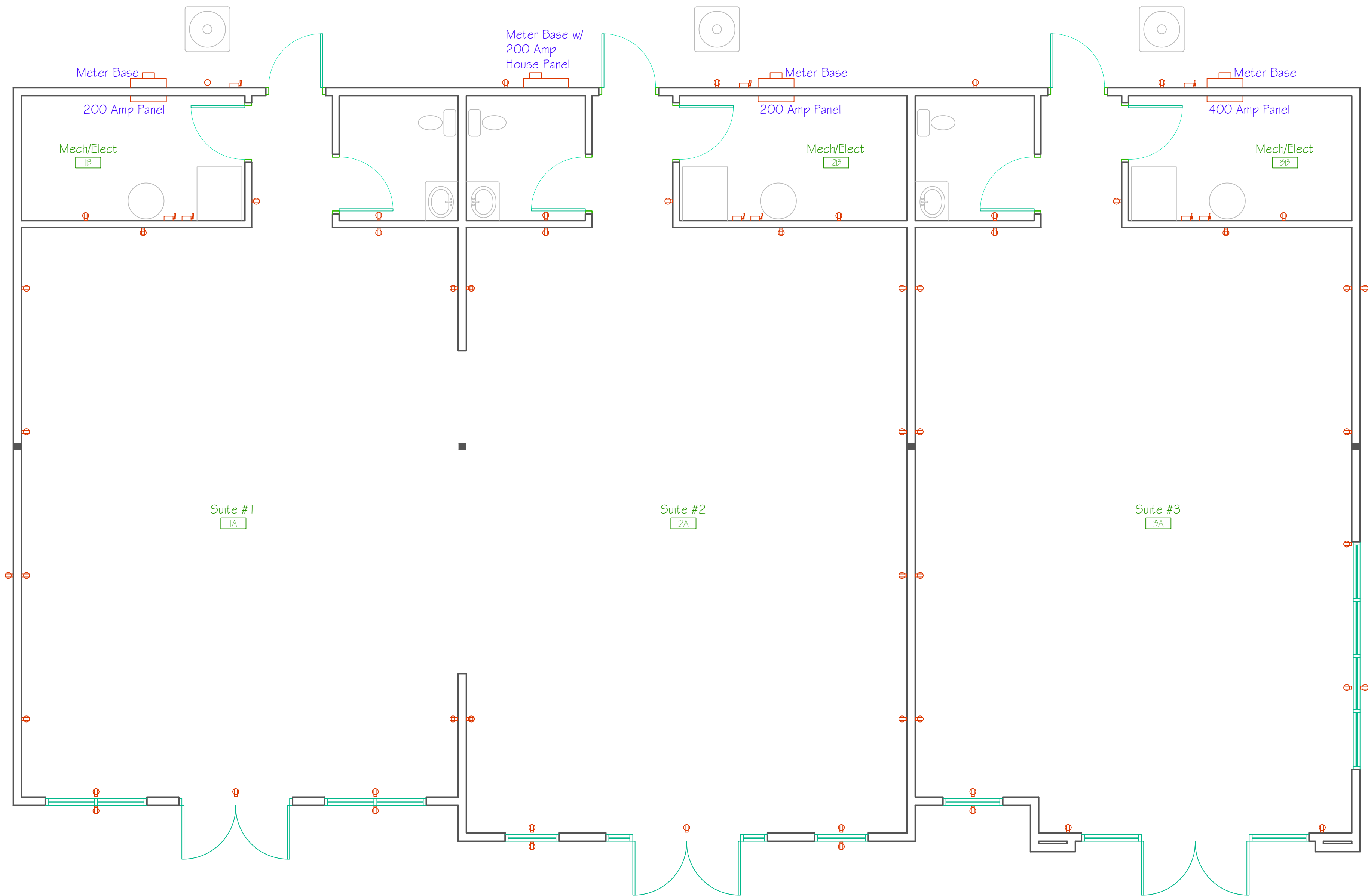
Power Plan
