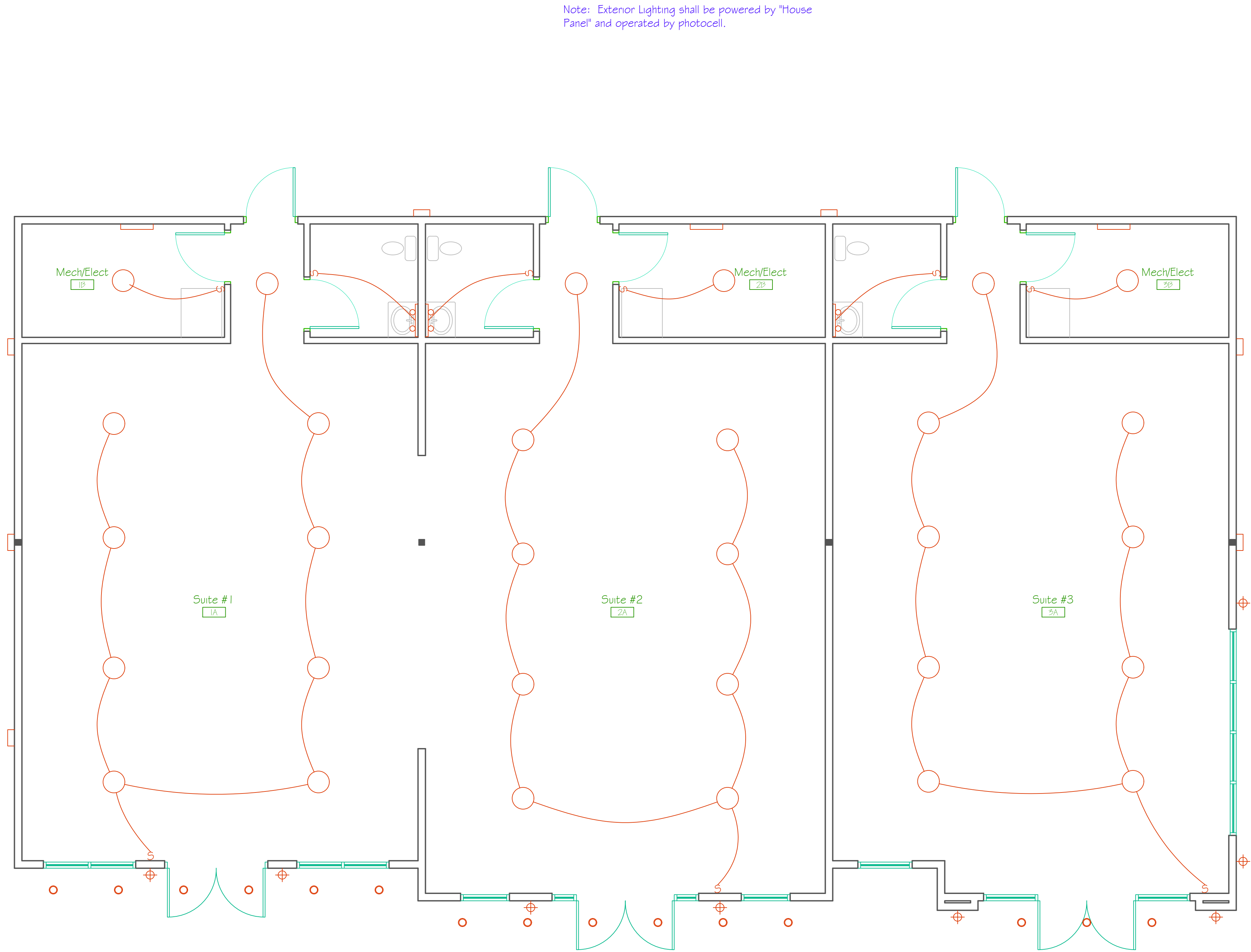
Lighting Plan
