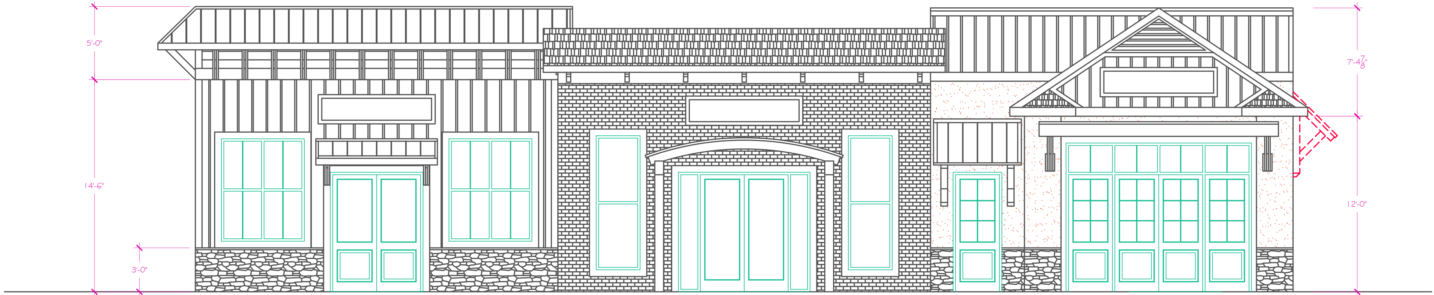
Front Elevation
