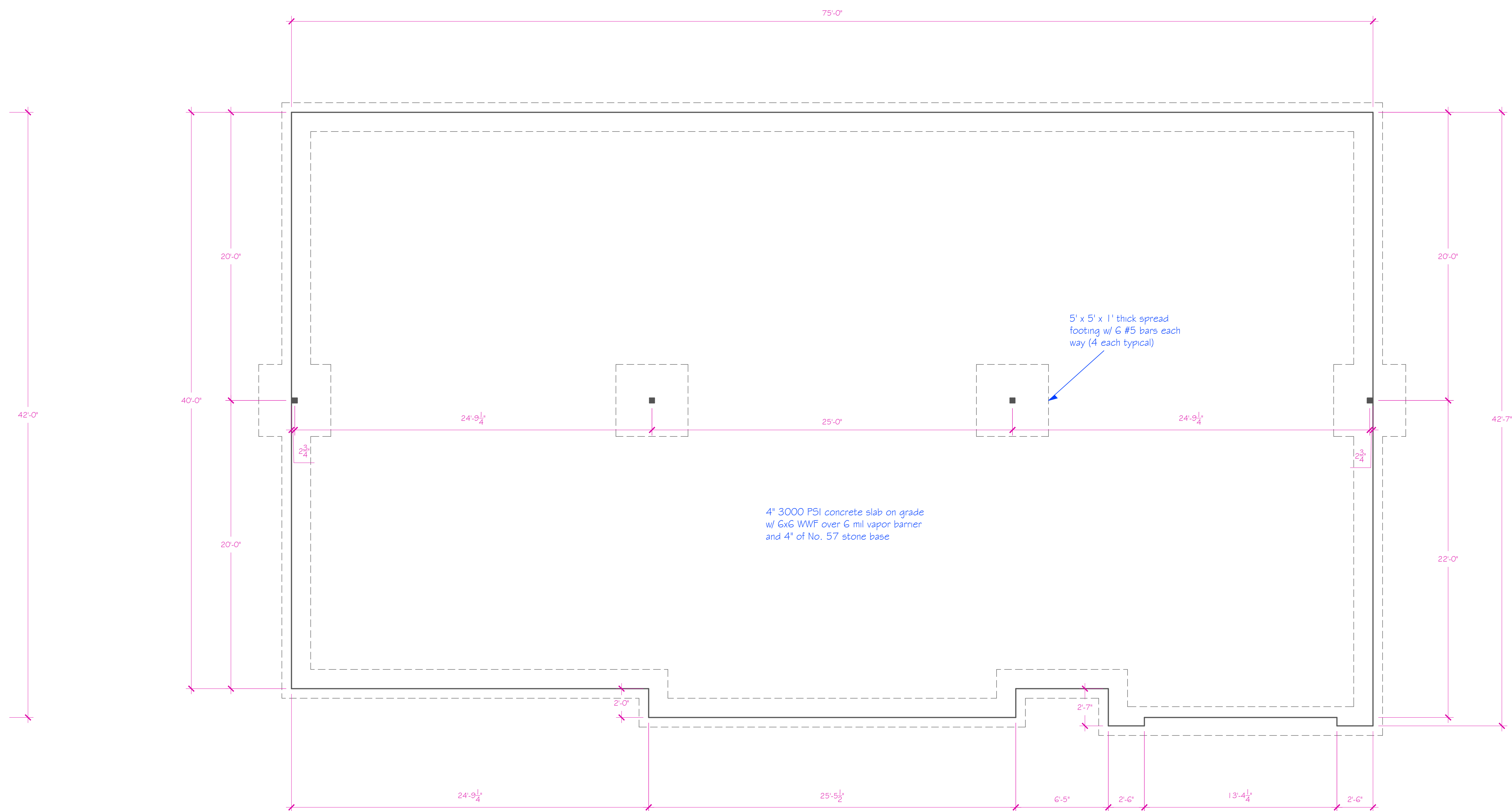
Foundation Plan
